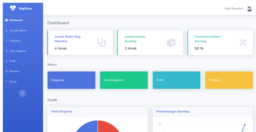
Gambar 3.4 Halaman Dashboard
